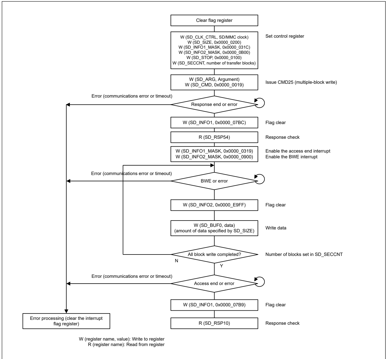
Figure 46.14 Example of multiple block write operation using internal timer
