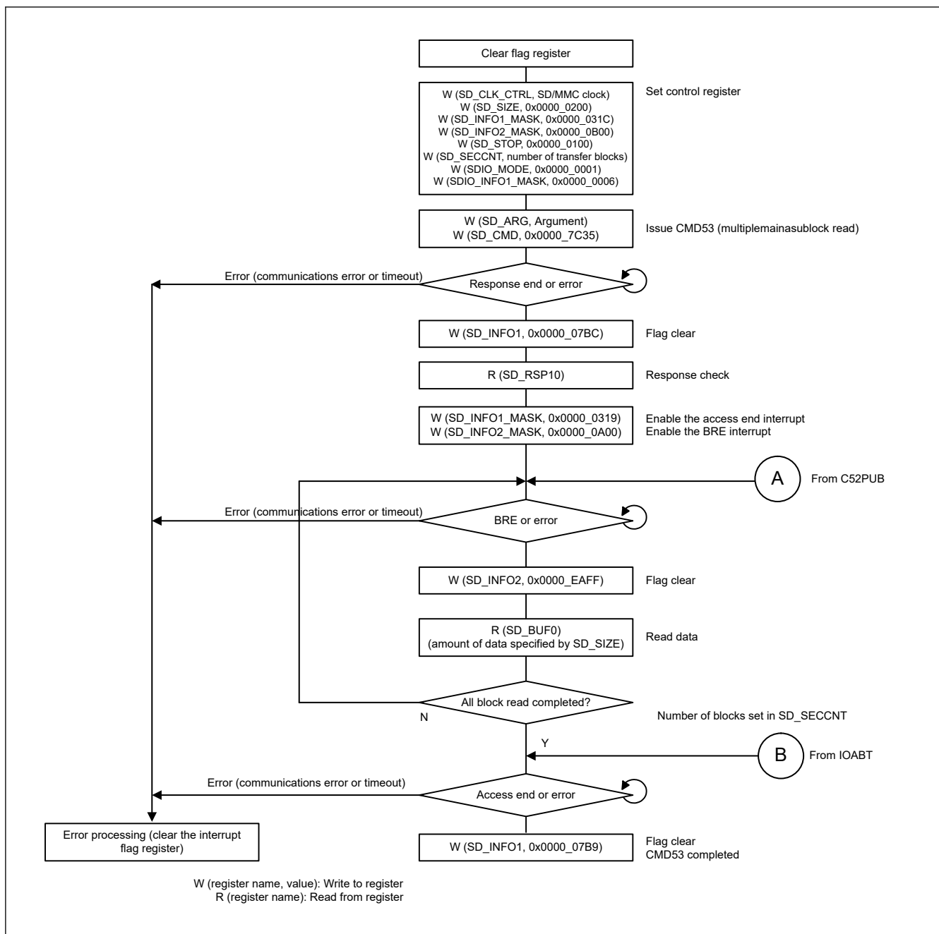
Figure 46.17 Example of IO_RW_EXTENDED command (CMD53) for multiple block read operation
