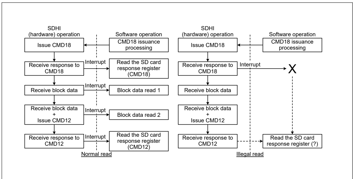
Figure 46.25 Multiple block read operation flow chart (two blocks)
