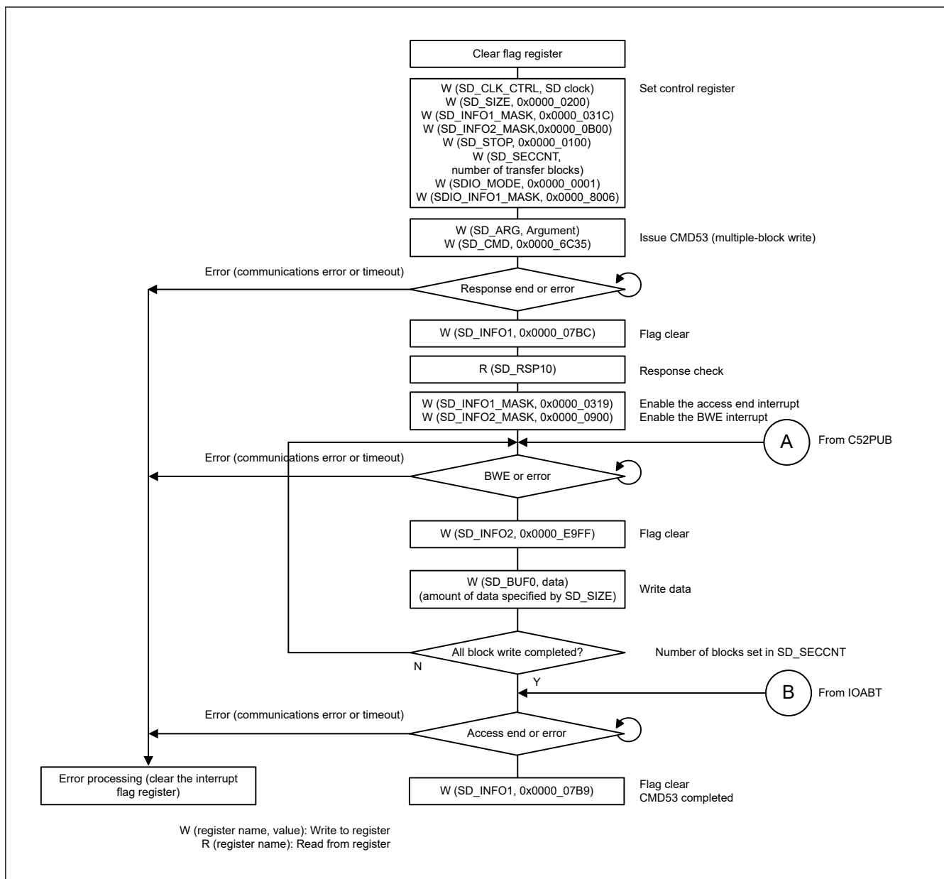
Figure 46.20 Example of IO_RW_EXTENDED command during a CMD53 multiple block write operation
