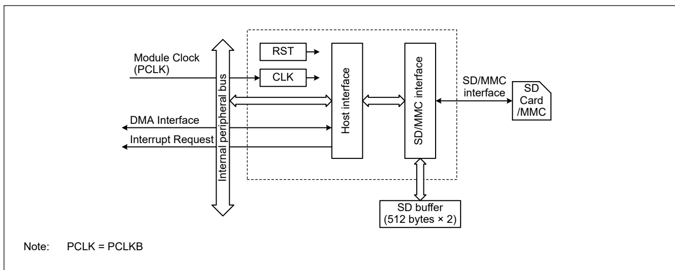
Figure 46.1 SD/MMC Host Interface block diagram
