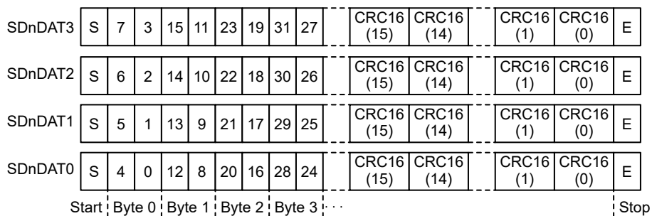
Figure 46.3 SDnDAT in 4-bit width mode
