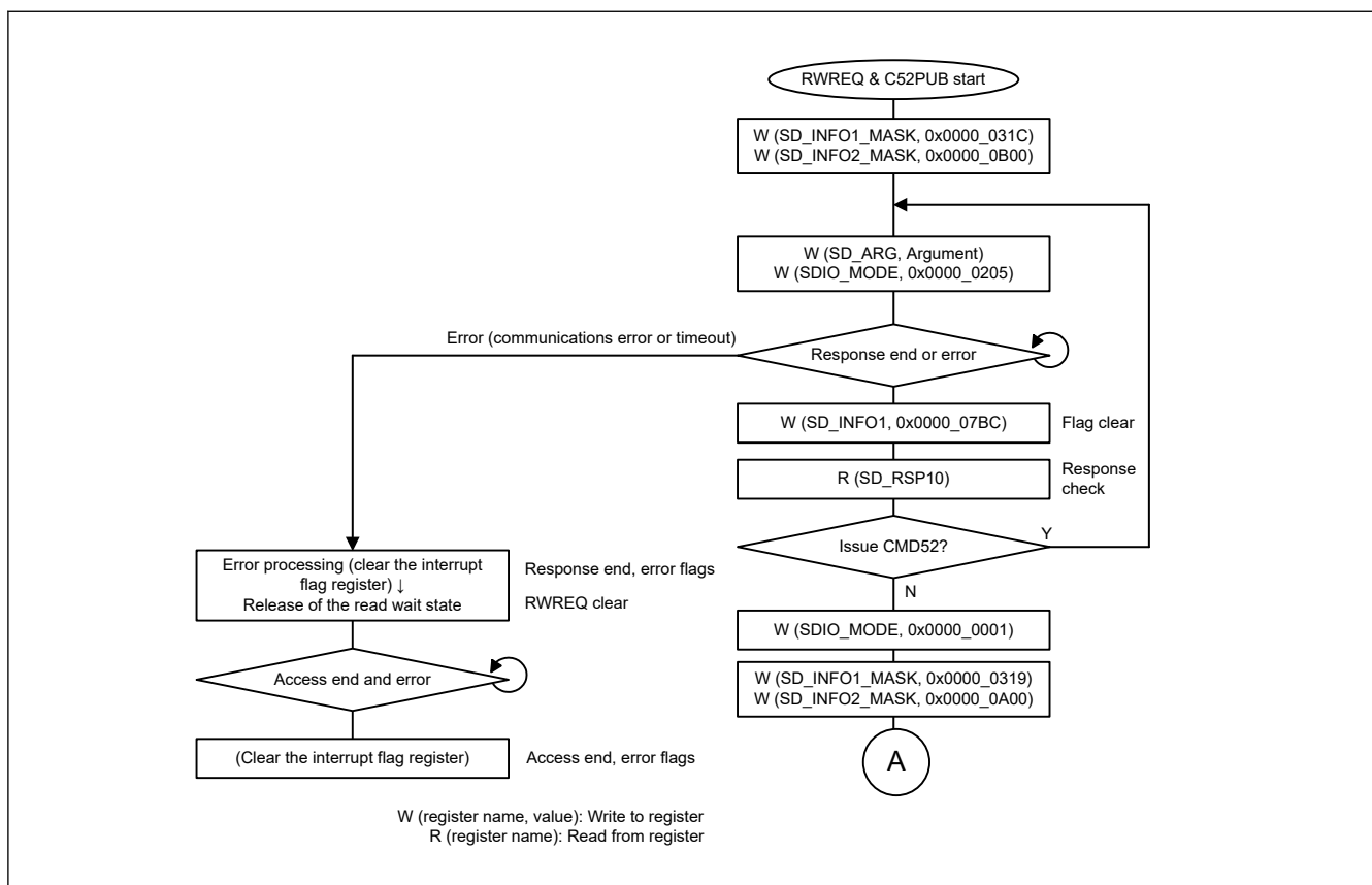
Figure 46.19 Flow when CMD52 (SDIO no abort) is issued during a CMD53 multiple block read while the SD Host Interface is in read wait state
